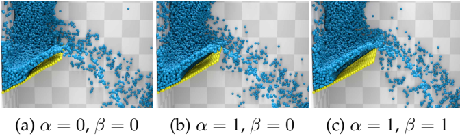
Fig. 10: Cross-section view of a simple solid-fluid coupling test, including a column of fluid falling onto an elastic cloth model, demonstrating the impact of different energy conservation parameters: (a) no energy preservation with \alpha = 0 and \beta = 0 , (b) full energy preservation for merging using \alpha = 1 and no energy preservation with velocity synchronization using \beta = 0 , and (c) full energy preservation with \alpha = 1 and \beta = 1 .
