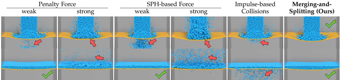
Fig. 4: Comparison of different methods for handling solid-fluid collisions: cross-section views of simulations including a soft elastic cloth hit by a fluid beam. Each column shows the same simulation at two different time steps. All particles have identical mass and weak/strong penalty and SPH-based force stiffness parameters differ by an order of magnitude. Notice that only our merging-and-splitting approach prevents penetrations without introducing instability.
