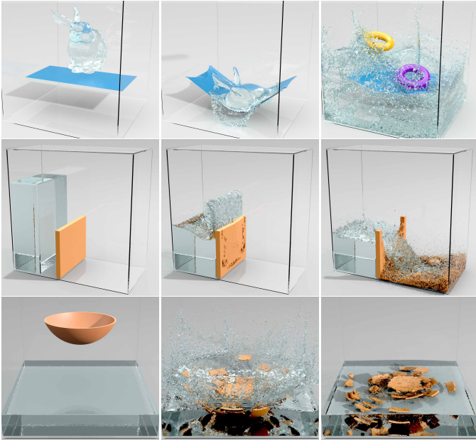
Fig. 8: Example frames from our simulation tests for coupling peridynamics and SPH using merging-and-splitting.
