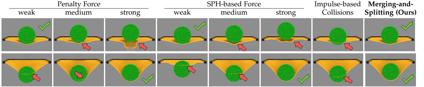
Fig. 3: Comparison of different methods for handling solid-solid collisions: cross-section views of simulations including a soft elastic cloth hit by a solid ball in free fall. The bottom row shows the same simulation with the solid ball falling from a higher initial position (i.e. faster impact). All particles have identical mass and weak/medium/strong penalty and SPH-based forces differ by an order of magnitude. Only our merging-and-splitting approach prevents penetrations without introducing instability for both cases.
