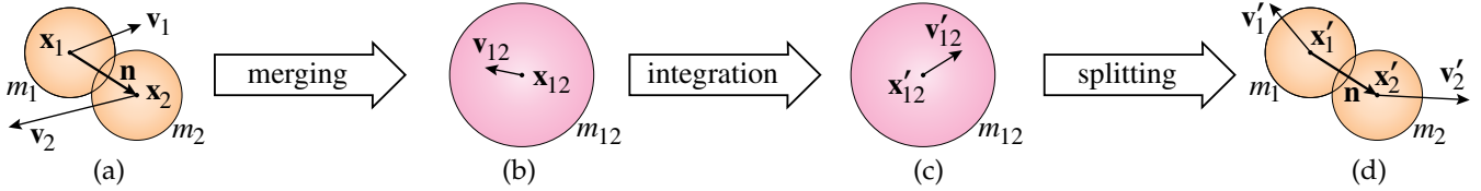
Fig. 1: The overview of merging-and-splitting approach: (a) colliding particles are merged into (b) a meta-particle using the principles of inelastic collision. This meta-particle is used during time integration to compute (c) its position and velocity at the end of the time-step. Finally, the meta-particle is split into (d) the two original particles with updated velocities, using the principles of elastic collision with momentum and energy conservation.
