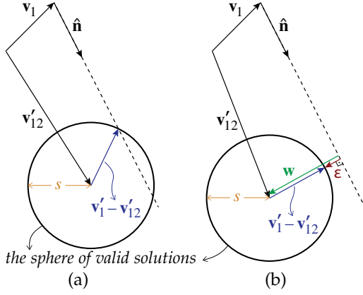
Fig. 2: Geometric solutions to the quadratic equation in Equation 13 showing the sphere of valid solutions centered around \mathbf{v}'_{12} that conserve momentum and energy: (a) quadratic equation has roots, and (b) quadratic equation has no real roots.
