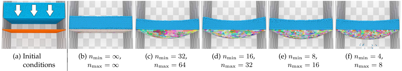
Fig. 11: A block of fluid falling with gravity onto a soft elastic cloth: (a) the initial conditions before the collision and (b-f) the simulation state a few seconds after the collision, comparing different parameters for n_{\min} , and n_{\max} that limit the number of particles in a meta-particle. Cloth particles having the same color are merged into the same meta-particle. Notice that (b) using an unlimited number of particles in a meta-particle with n_{\min} = n_{\max} = \infty leads to rigidification and (f) using too small limits causes leaks.
