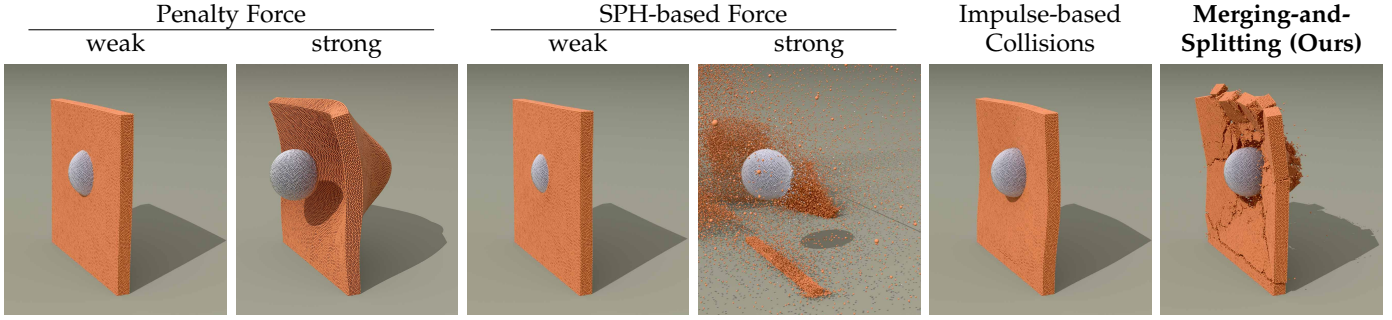
Fig. 5: Comparison of different methods for collision handling in fracture simulation: a solid brittle wall is hit by a dense ball with 20\times heavier particles. The bottom row shows the same simulation from a different view at a later time step. Notice that only our merging-and-splitting approach can produce a stable fracture simulation with pleasing result.
